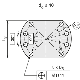
Drilling pattern 2
