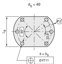
Drilling pattern 1
