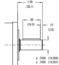
NemaTRUE PLUS* (NTP) HeavyDuty Output Shaft
