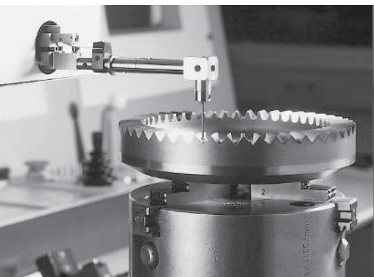
Computerized mapping of gear tooth profile
