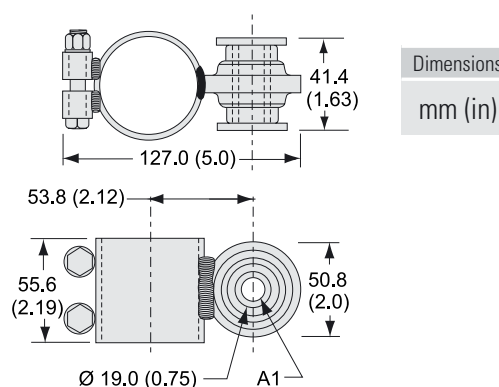
Electrak PPA Tube Mount - Heavy-duty 6670 N (1500 lbf)
